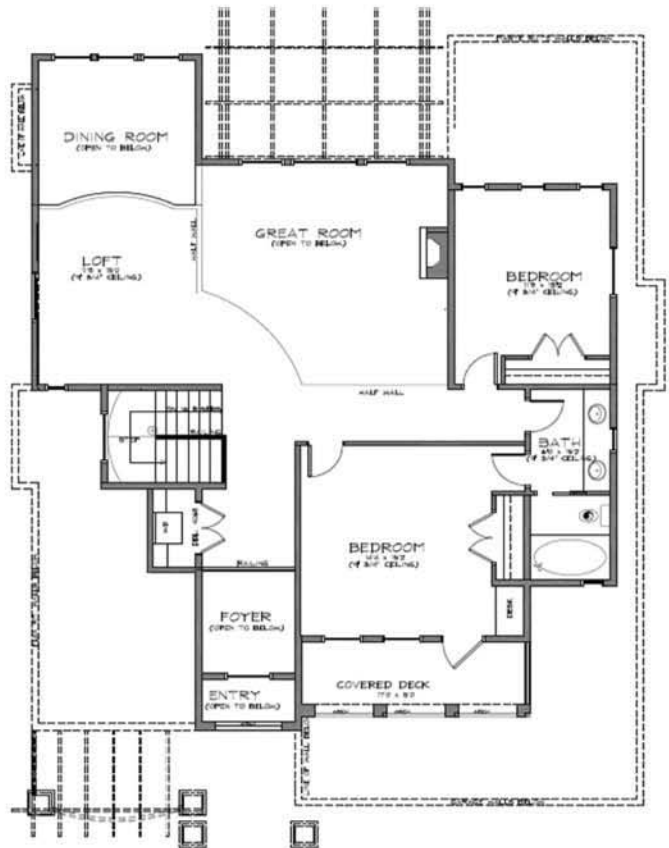
Upper Floor Plan 998 sq. ft.
