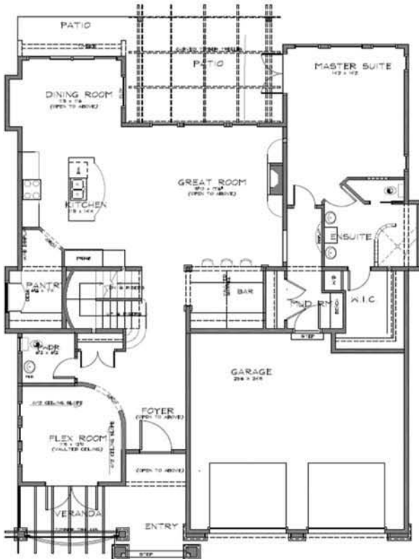
Main Floor Plan 1867 sq. ft.
