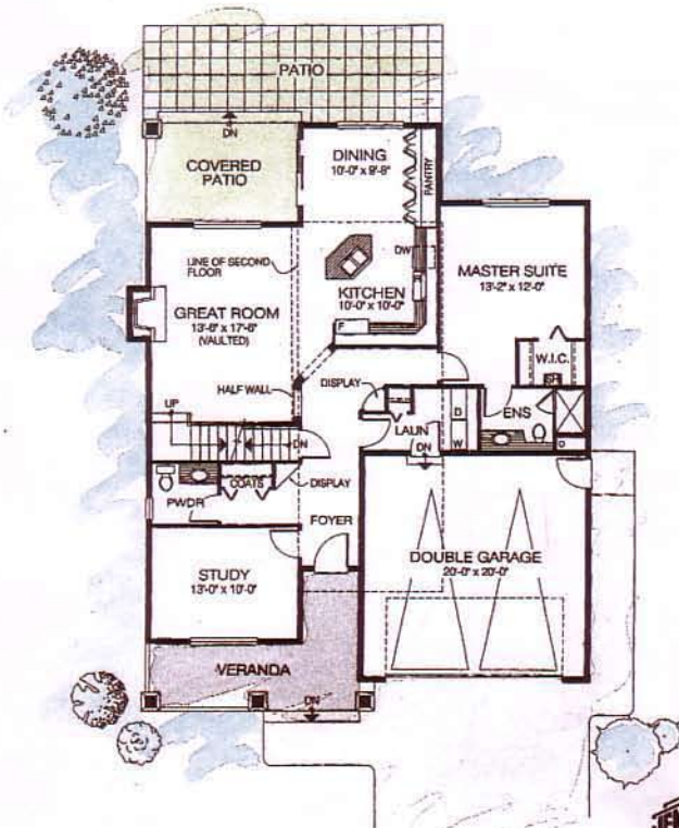
MAIN FLOOR PLAN 1238 SQ. FT. (119.2 M 2 )
