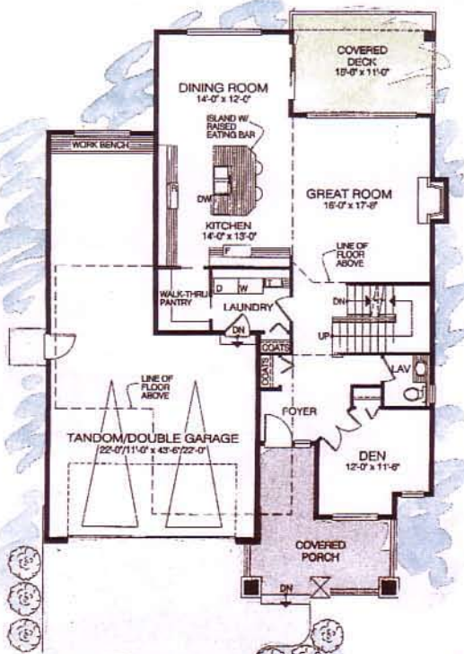
MAIN FLOOR PLAN 1195 SQ. FT. (111.0 M 2 )
